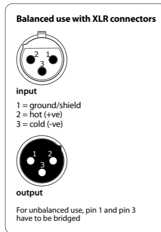
Fig. 8.2: Conector XLR
